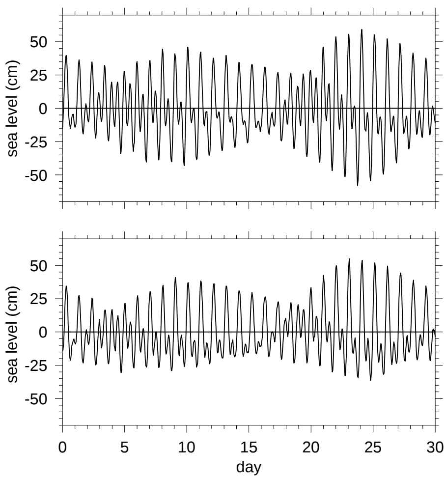
Plate12: Hilo and Honolulu sea level, May 1990
