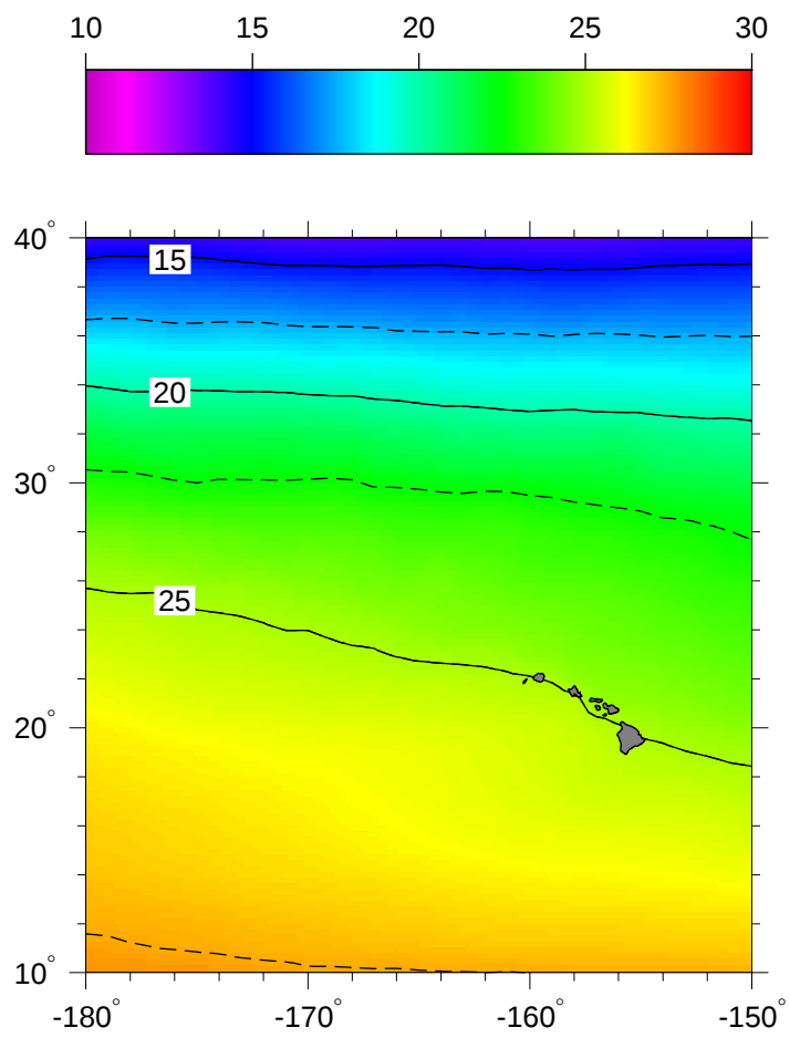
Plate 3b: spring temperature field
