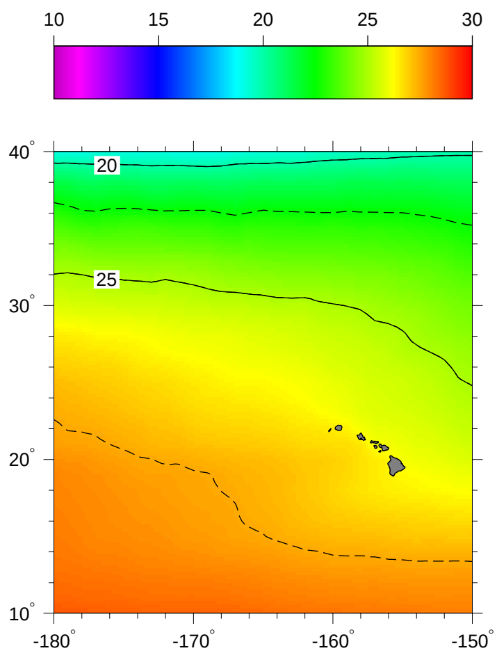
Plate 3c: summer temperature field
